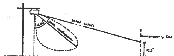
Type 3: Luminaire with less than 90 degree cutoff
